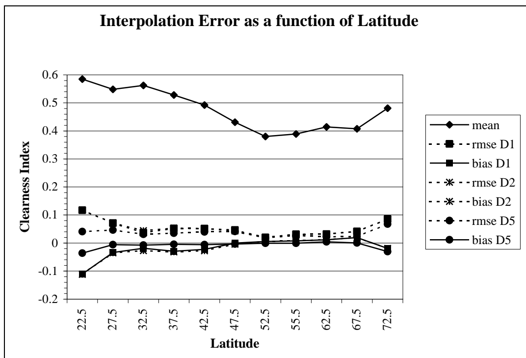
Figure 1. Interpolation errors (bias, RMSE) as a function of the latitude (in degrees) for the cleanness index, using three different distances D1 , D2 and D5 and the gravity method. The mean value of the measured cleanness index is also given.
